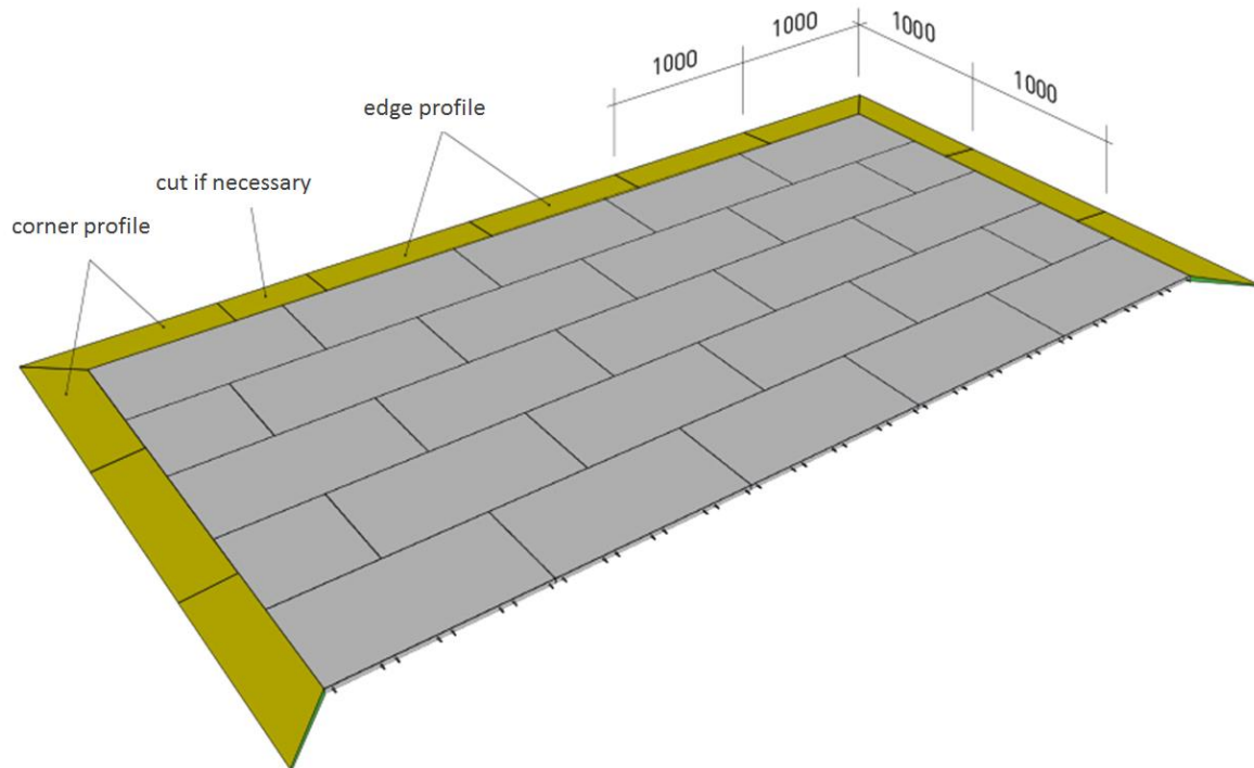
Installation of the profiles
